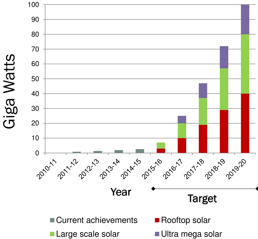
India: Total Solar PV Capacity and Targets
